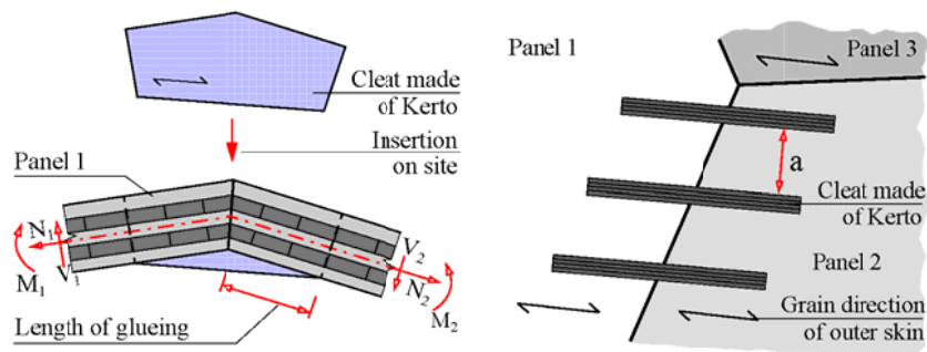
Figure 4. The "sewed" joints, left : cross section showing axial forces N_1 resp. N_2 , lateral forces V_1 resp. V_2 and bending moments M_1 resp. M_2 , right : top view.
